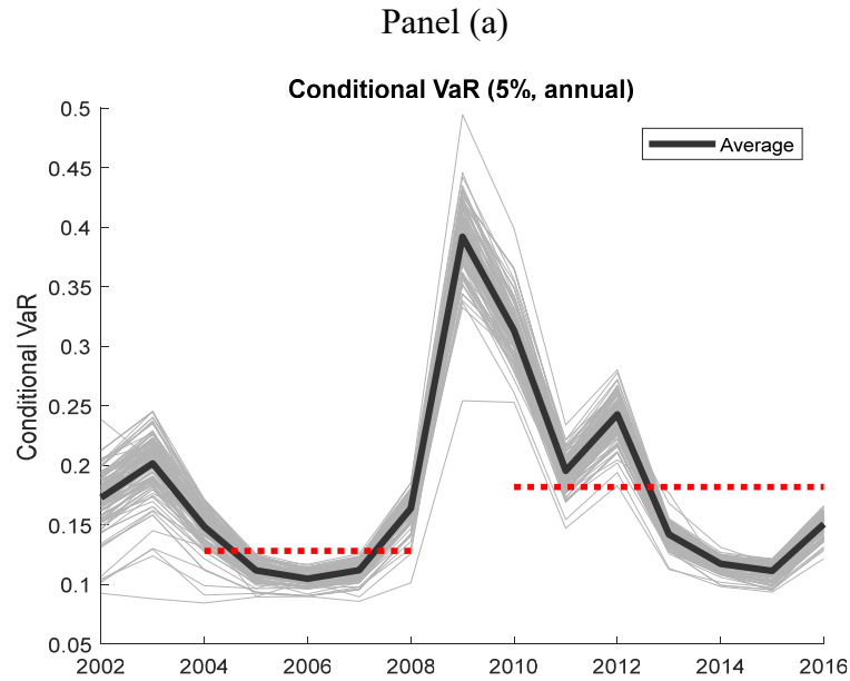
Figure 6. VaR-based measures of risk
